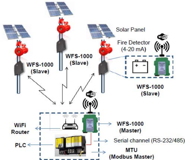
Figure 2.- Typical WFS-1000 application as Modbus RTU
