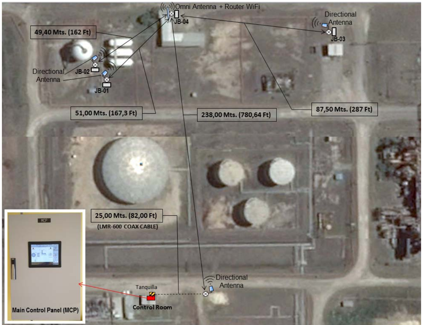
Figure 3.- WiFi Sentinel deployed on field
