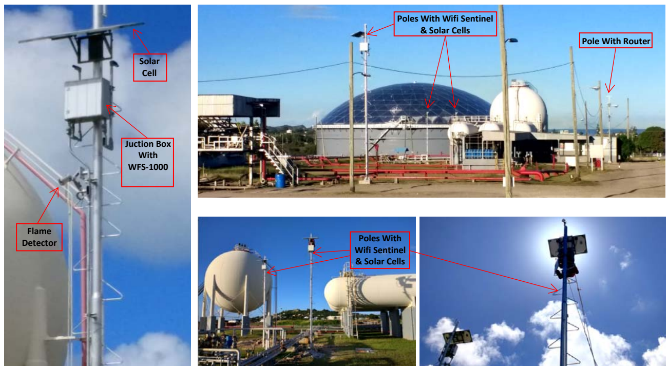
Figure 2.- WiFi Sentinel in a real application
