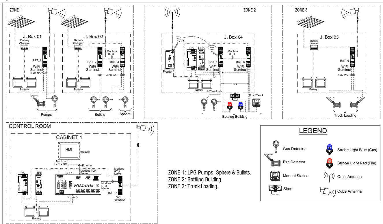
Figure 1.- WiFi Sentinel System Architecture
